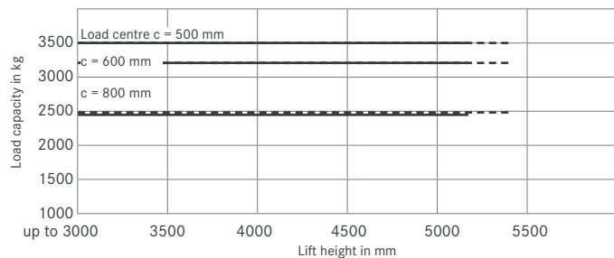
RX 60-35 Telescopic/HiLo mast
