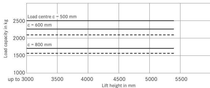
RX 60-25 Telescopic/HiLo mast
