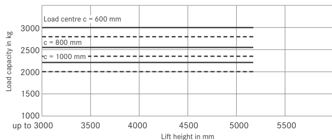
RX 60-30/600 Telescopic/HiLo mast
