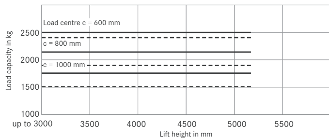
RX 60-25/600 Telescopic/HiLo mast
