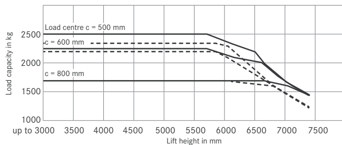
RX 60-25 triplex mast
