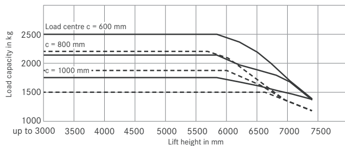
RX 60-25/600 triplex mast
