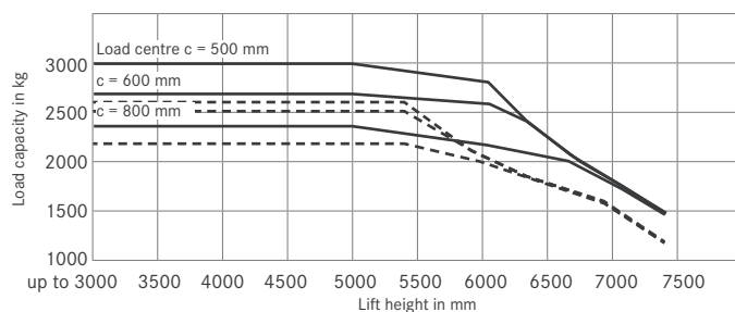
RX 60-30 triplex mast
