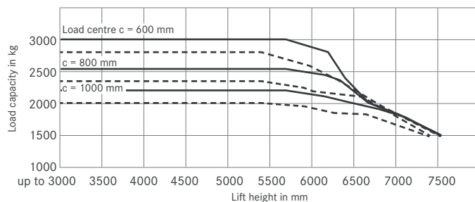
RX 60-30/600 triplex mast
